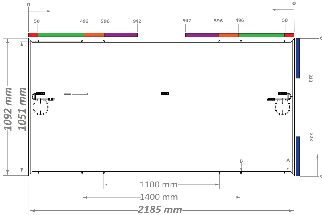
A - Ground Holes (4X Ø 4.2mm) B - Mounting Holes (8X 9mm (W) x 14mm (L), R4.5mm)
