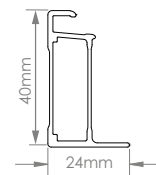
END FRAME PROFILE
