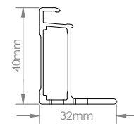
SIDE FRAME PROFILE
