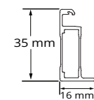
END FRAME PROFILE
