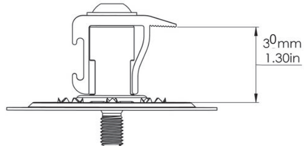
PVKIT Grab's Acceptable Module Thickness Range
