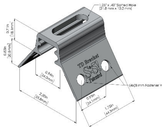
TD Bracket
