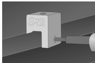
Step 3: Tighten to correct torque
