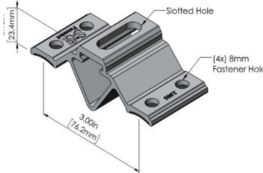
CorruBracket™ 500T
