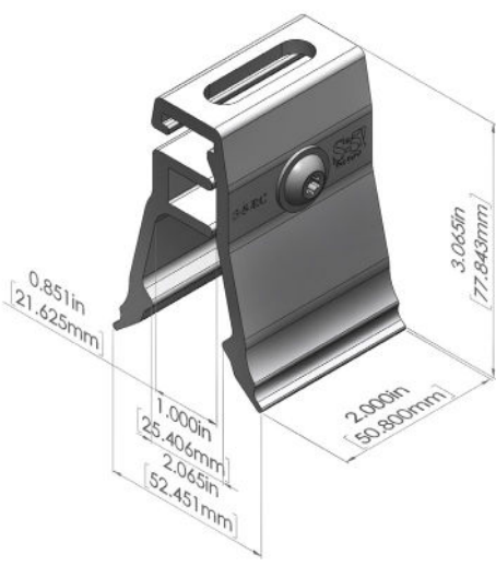
S-5-RC™
