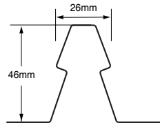
Conceal Fix Tall S-5-HR
