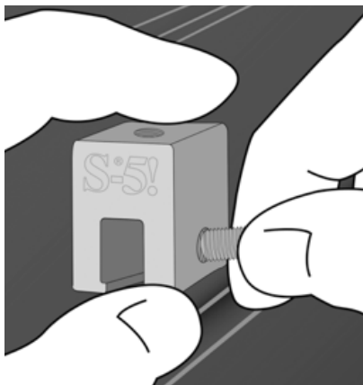
Step 1: Preload setscrews
