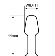
44mm Bulb Seam EU S-5-Z, S-5-Z Mini S-5-R465, S-5-R465 Mini Clamp choice dependent on bulb width
