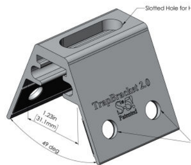
TrapBracket™ 2.0
