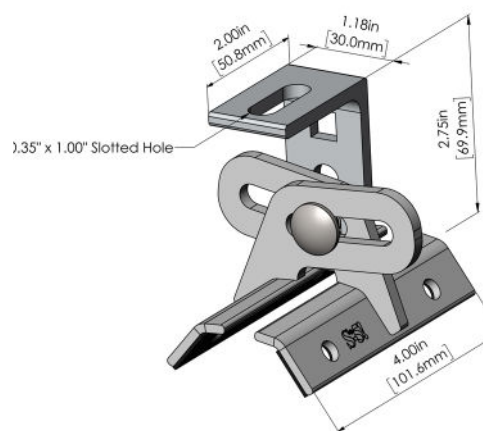
ProteaBracket™
